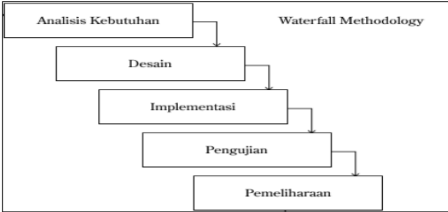
Gambar 2.2 Metode Waterfall
