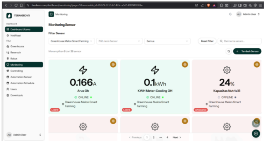
Gambar 2.1 Website ITERAHERO
